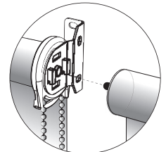
Shared Bracket
