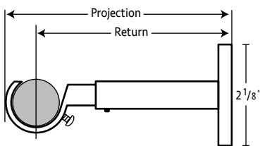
Extendible Single Bracket
