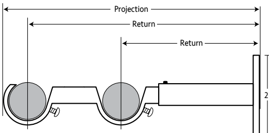
Extendible Double Bracket
