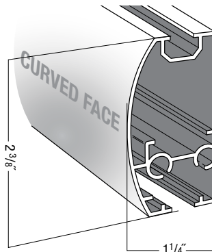
Coimbra Track with Curved Face to Front
