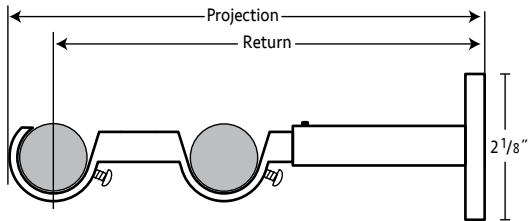
Extendible Basic Double Bracket
