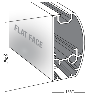
Coimbra Track with Flat Face to Front
