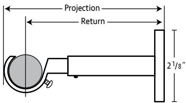
Extendible Basic Single Bracket
