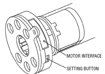
Motor Head for Wand Controlled Motor
